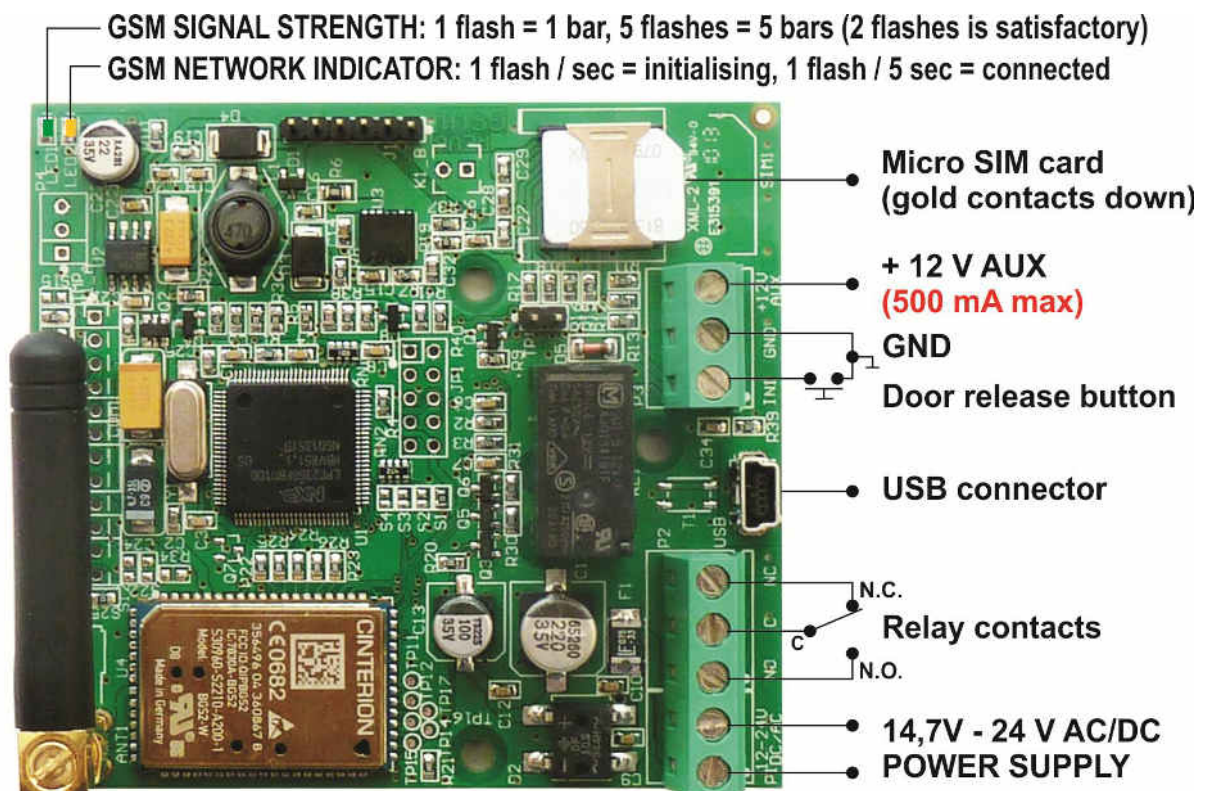
Figure 1: GSW1 Connection diagram
